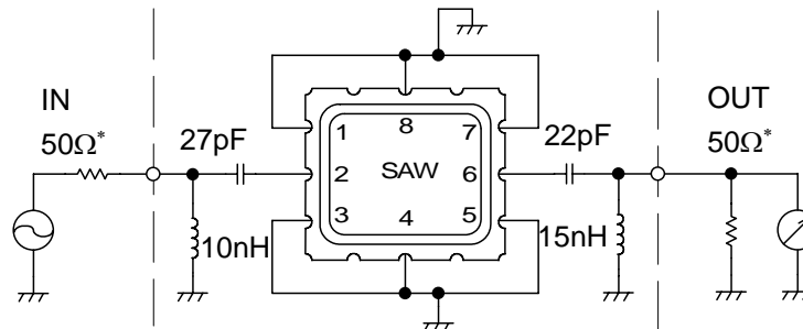
Fig.1 Measuring Circuit
